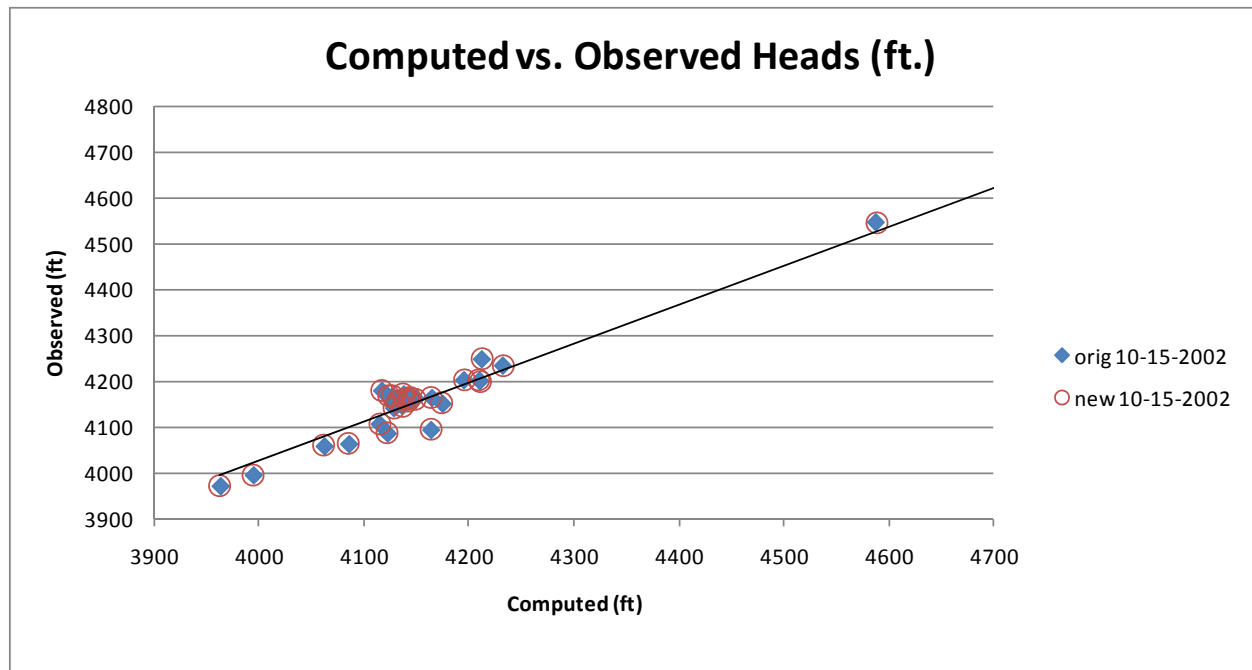
FIGURE 6. COMPUTED VS. OBSERVED HEADS (FT.) FOR OCTOBER 15, 2002 FOR THE ORIGINAL USGS MODEL (POOL AND DICKINSON, 2007) AND AFTER CORRECTIONS TO MODEL.
