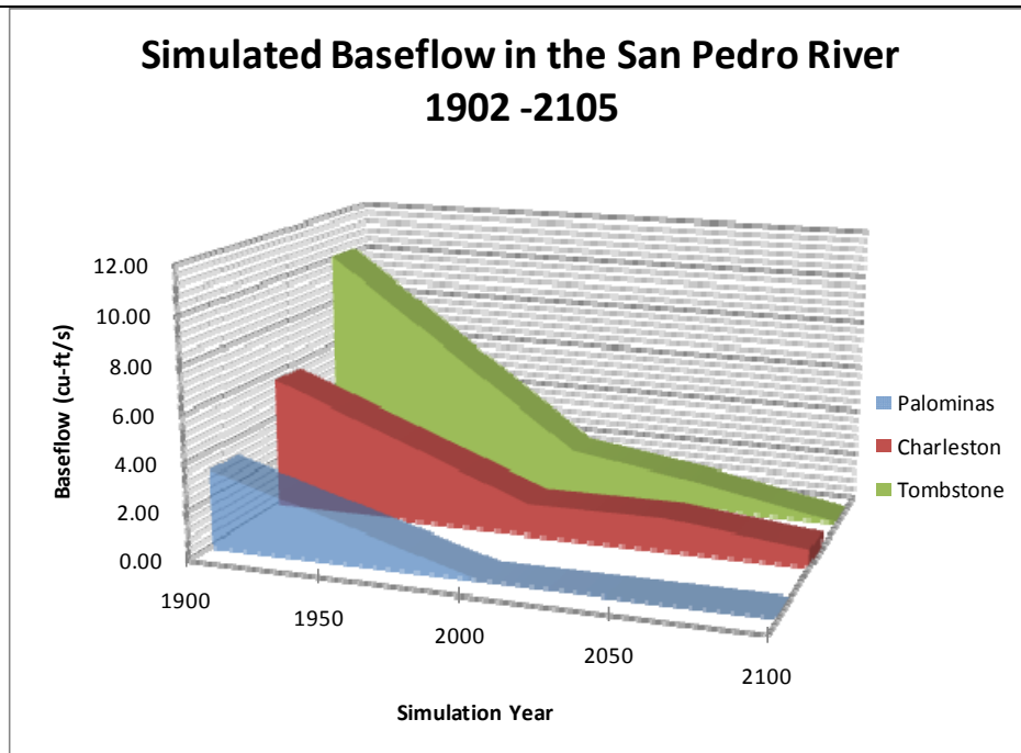
FIGURE 22. SIMULATED OCTOBER BASEFLOWS (CU-FT/S) IN THE SAN PEDRO RIVER AT THE PALOMINAS, CHARLESTON, AND TOMBSTONE GAGING STATIONS IN 1902, 2000, 2050, AND 2100.
