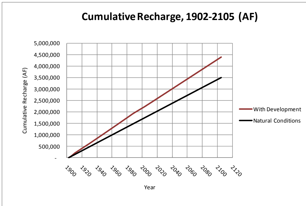
FIGURE 17. SIMULATED CUMULATIVE TOTAL RECHARGE (AF) WITH AND WITHOUT HUMAN DEVELOPMENT, 1902-2105.
