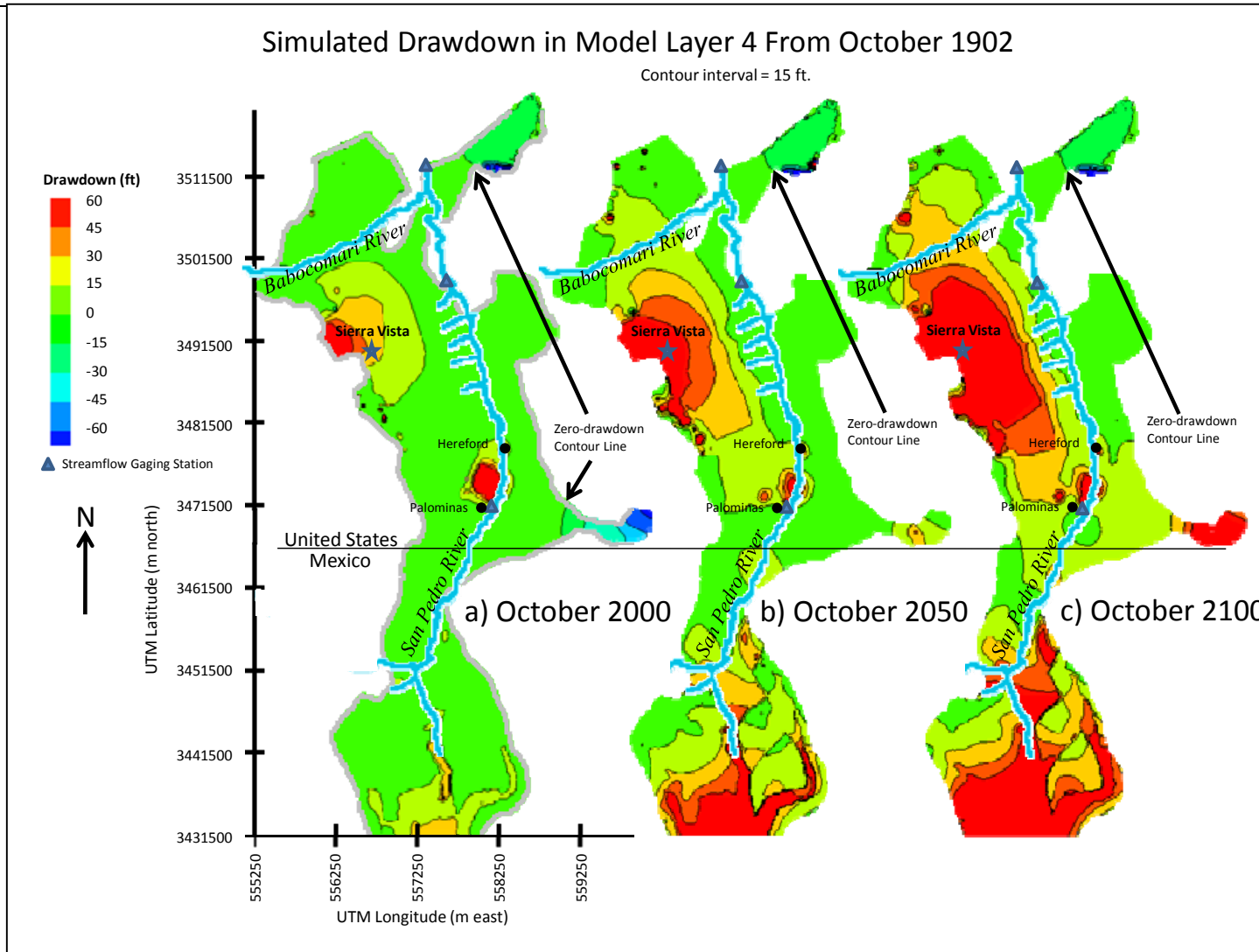
FIGURE 18. SIMULATED CHANGE IN HEAD (DRAWDOWN) (FT.) IN MODEL LAYER 4 (REGIONAL BASIN-FILL AQUIFER) FROM OCTOBER 1902 TO OCTOBER 2000, OCTOBER 2050, AND OCTOBER 2100. AREAS IN DARK RED REPRESENT DRAWDOWN OF 60 FT. OR MORE. BLUE LINE REPRESENTS LOCATION OF RIVERS BUT DOES NOT SIGNIFY THE CONDITION OF PERENNIAL FLOW.
