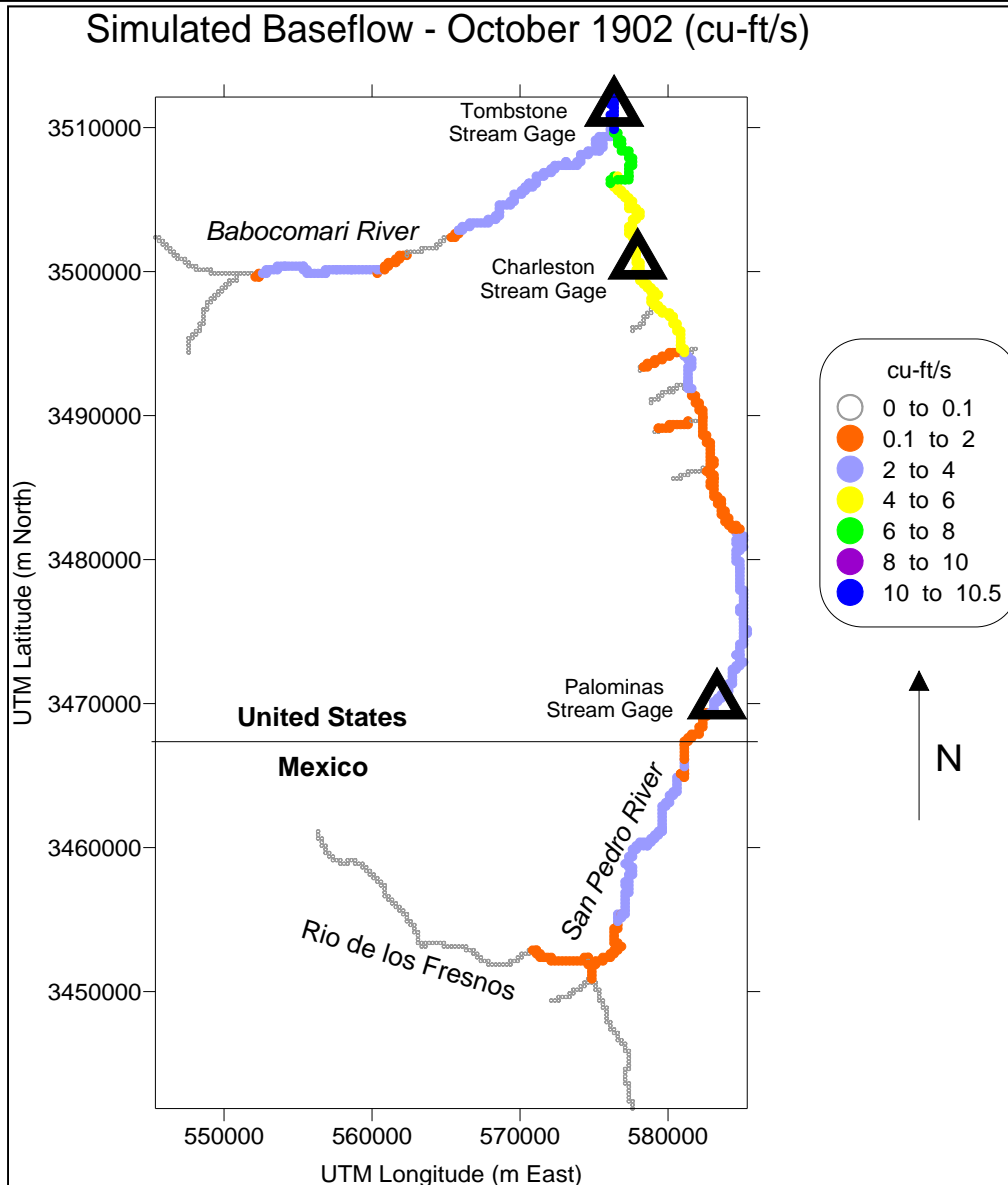
FIGURE 20. SIMULATED BASEFLOW FOR OCTOBER 1902 (CU-FT/S).
