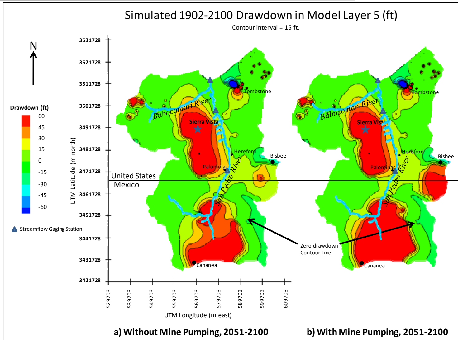
FIGURE 27. SIMULATED DRAWDOWN (FT.) FROM 1902 TO 2100 IN MODEL LAYER 5: A) WITHOUT MINE PUMPING FROM 2051-2100, AND B) WITH MINE PUMPING FROM 2051-2100. THE “WITH MINE PUMPING” SCENARIO IS THE SAME AS THE PROJECTED DEVELOPMENT MODEL DESCRIBED IN THIS STUDY AND PRESENTED IN FIGURE 19(C).
