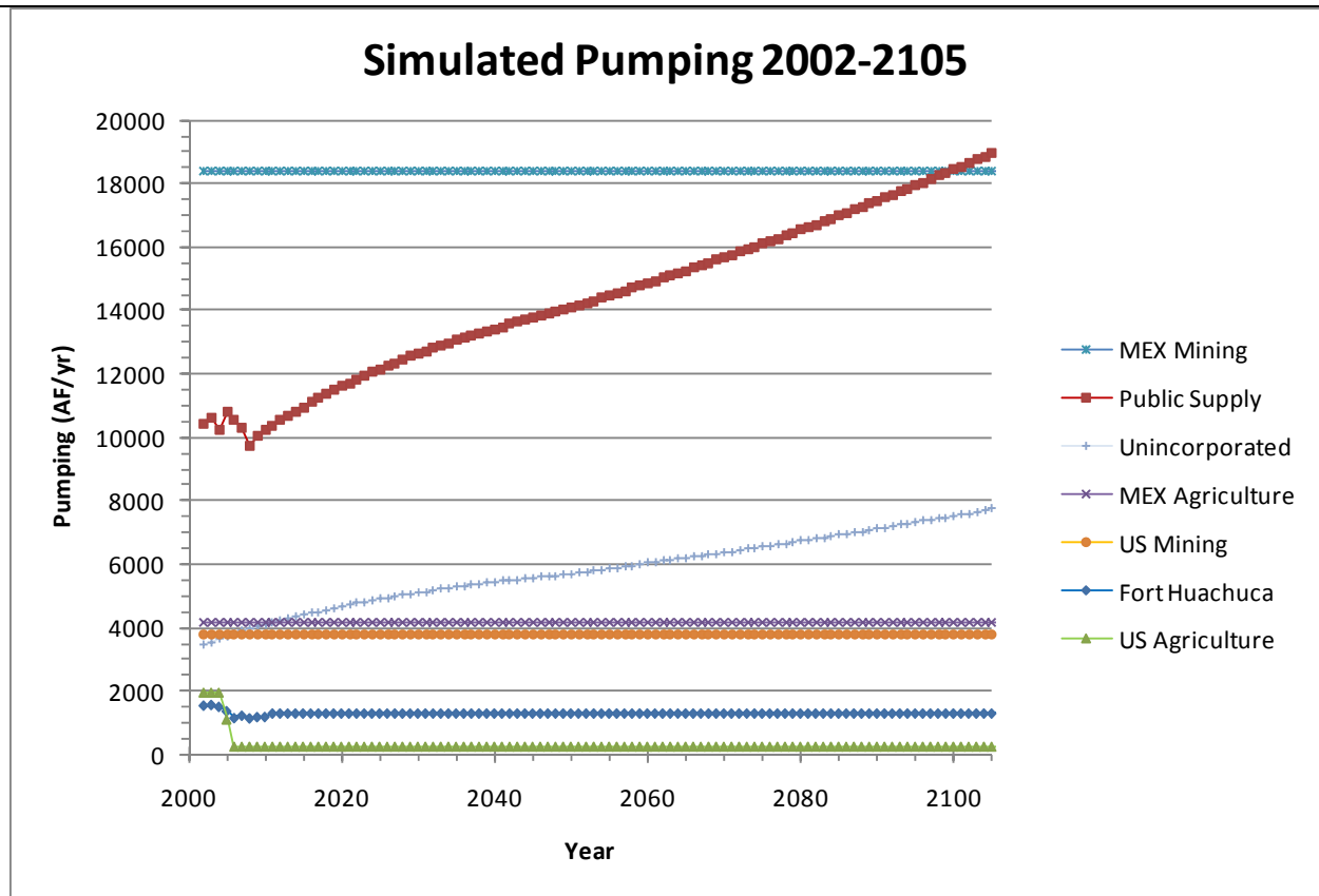
FIGURE 10. SIMULATED PUMPING RATES (AF/YR) FOR 2002-2105 PARTITIONED BY TYPE OF USE AND COUNTRY.
