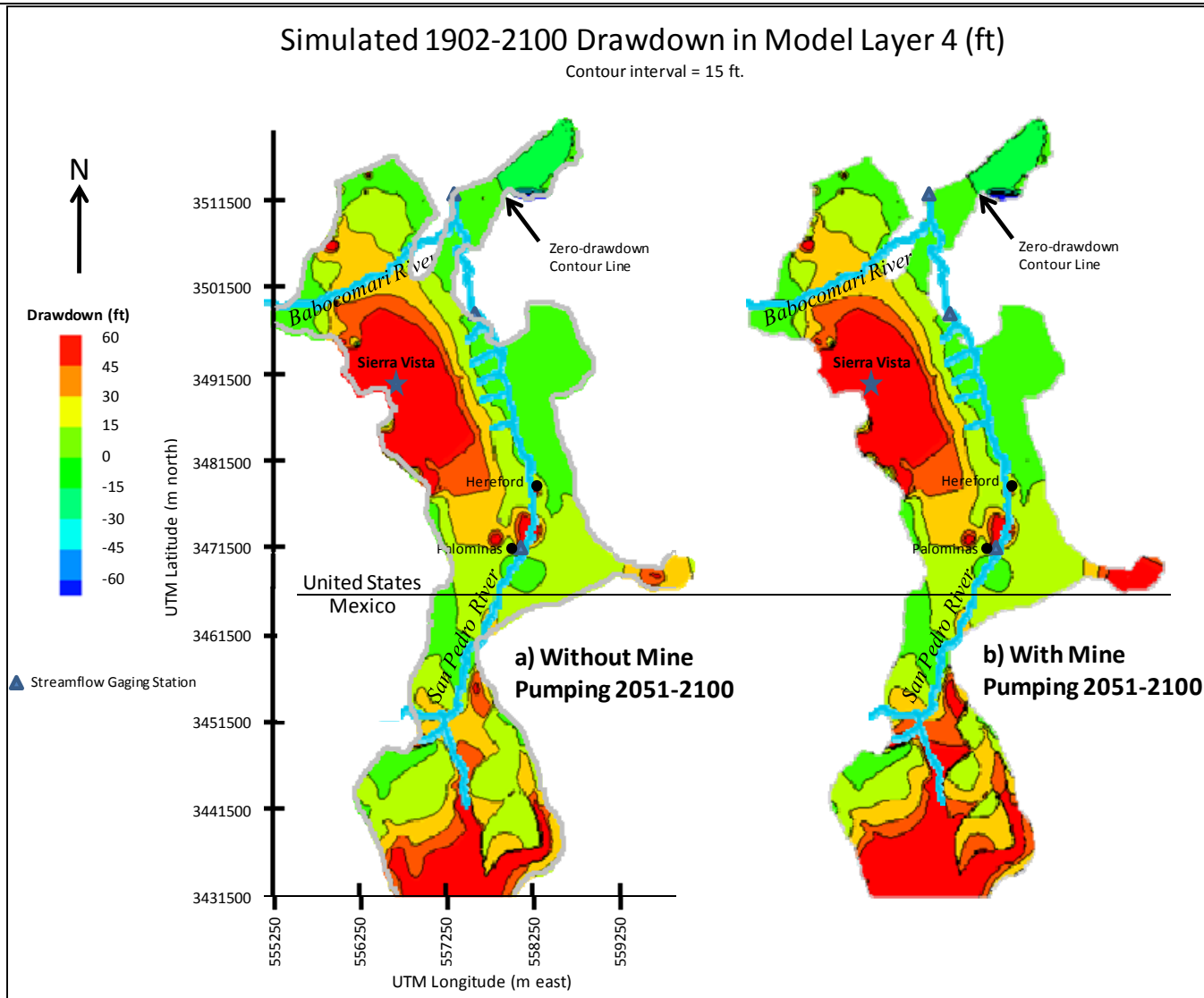
FIGURE 26. SIMULATED DRAWDOWN (FT.) FROM 1902 TO 2100 IN MODEL LAYER 4: A) WITHOUT MINE PUMPING FROM 2051-2100, AND B) WITH MINE PUMPING FROM 2051-2100. THE “WITH MINE PUMPING” SCENARIO IS THE SAME AS THE PROJECTED DEVELOPMENT MODEL DESCRIBED IN THIS STUDY AND PRESENTED IN FIGURE 18(C).
