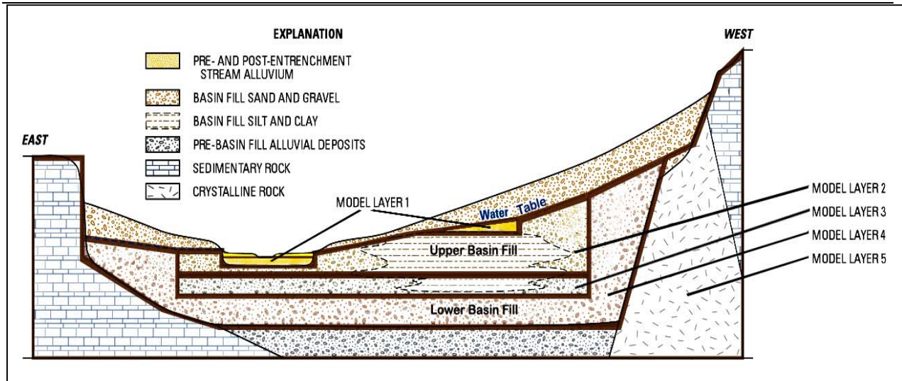
FIGURE 3. CONCEPTUALIZED CROSS SECTION OF USPB SHOWING MODEL LAYERS (FROM FIGURE 3 IN POOL AND DICKINSON (2007)).
