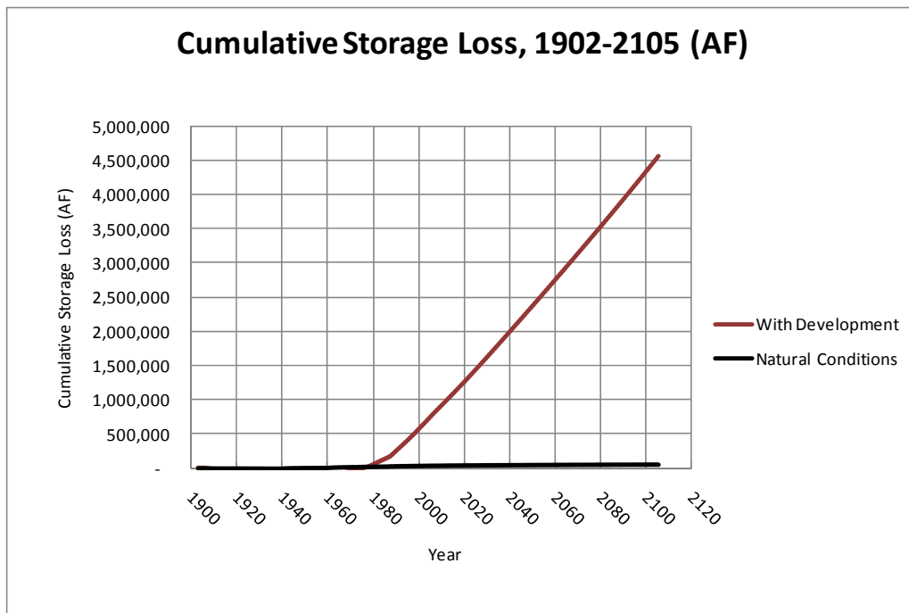
FIGURE 15. SIMULATED CUMULATIVE AQUIFER STORAGE (AF) LOSS WITH AND WITHOUT HUMAN DEVELOPMENT FOR THE SIMULATION PERIOD 1902-2105.
