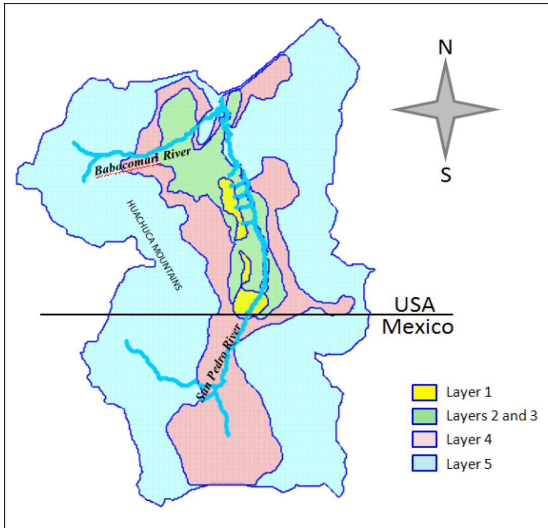
FIGURE 4. USBP MODEL LAYERS IN PLAN VIEW WITH SAN PEDRO RIVER INTERSECTING VARIOUS LAYERS. BLUE LINE REPRESENTS RIVER LOCATION BUT DOES NOT NECESSARILY SIGNIFY PERENNIAL FLOW CONDITION.
