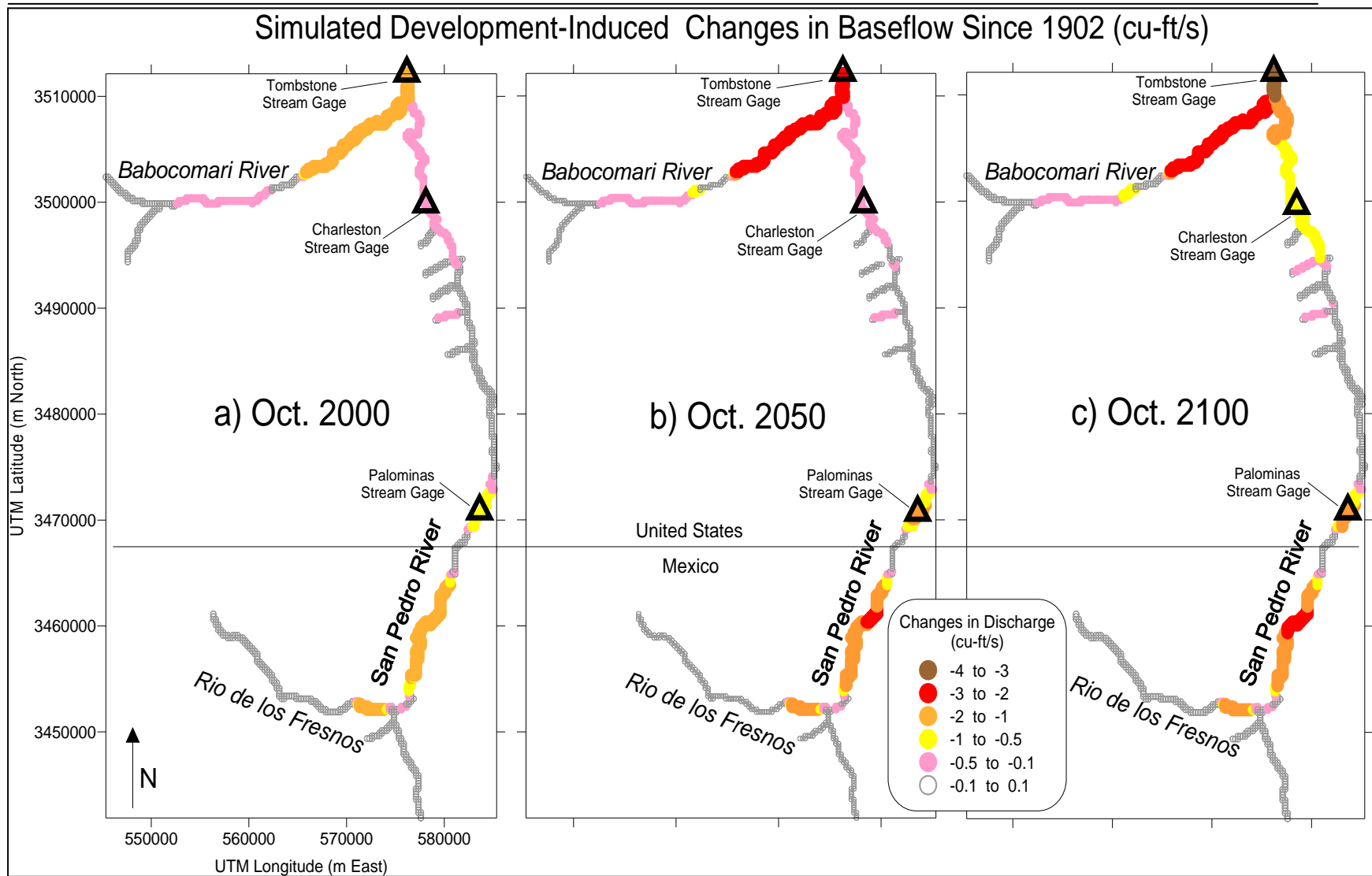
FIGURE 23. SIMULATED CHANGES IN STREAM BASEFLOW (CU-FT/S) ATTRIBUTABLE TO HUMAN DEVELOPMENT FROM 1902 TO: A) OCTOBER 2000, B) OCTOBER 2050, AND C) OCTOBER 2100. NEGATIVE CHANGE IN DISCHARGE CORRESPONDS TO DECLINING FLOW.
