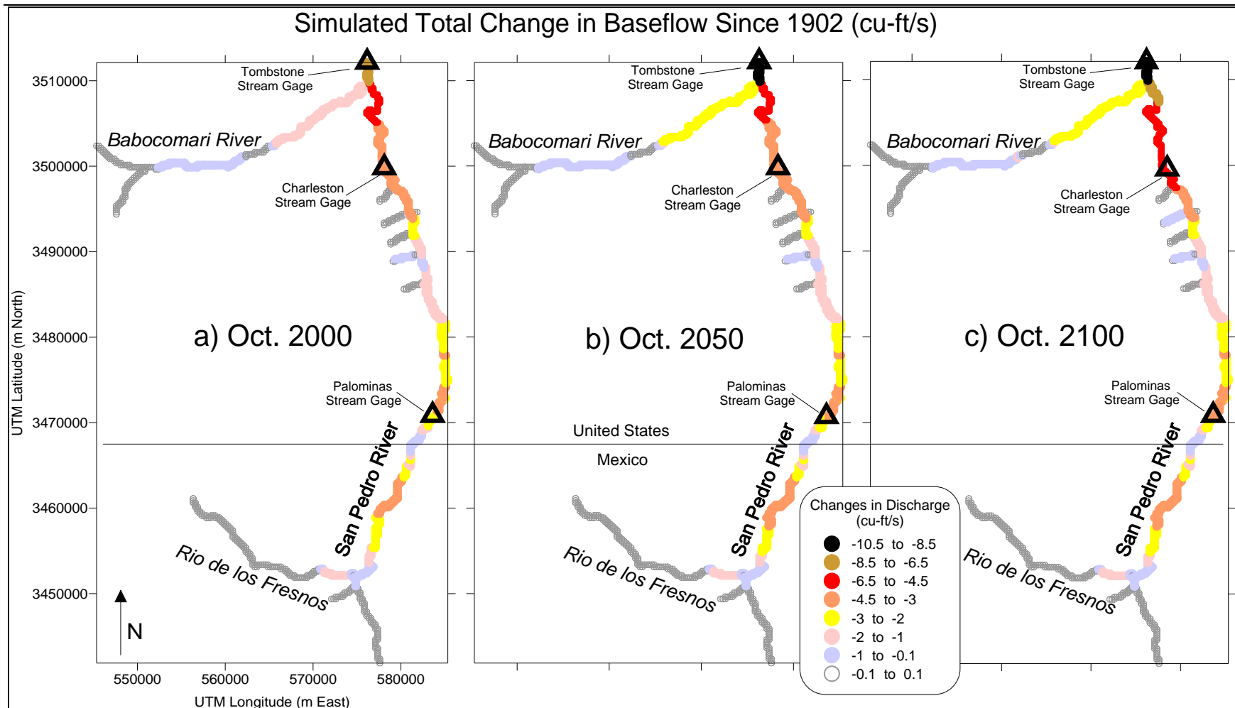
FIGURE 21. SIMULATED TOTAL CHANGE IN BASEFLOW FROM OCTOBER 1902 TO: A) OCTOBER 2000, B) OCTOBER 2050, AND C) OCTOBER 2100 (CU-FT/S). TOTAL CHANGE IN BASEFLOW INCLUDES CHANGES DUE TO ALL HUMAN AND NATURAL CAUSES, INCLUDING PUMPING, EVAPOTRANSPIRATION, AND RECHARGE.
