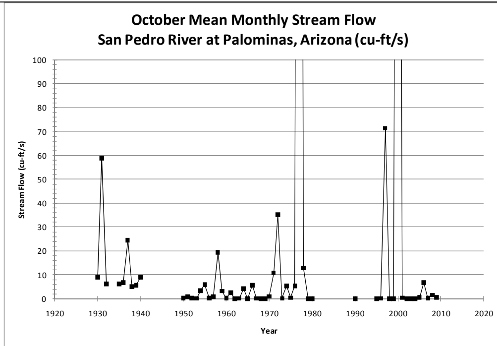
FIGURE 8. MEAN OCTOBER STREAM FLOW (CU-FT/S) MEASURED ON THE SAN PEDRO RIVER AT THE PALOMINAS GAGING STATION FOR THE PERIOD OF RECORD, 1920-2010 (USGS, 2011). VERTICAL AXIS IS TRUNCATED AT 100 CU-FT/S TO HIGHLIGHT LOW FLOWS. 9
