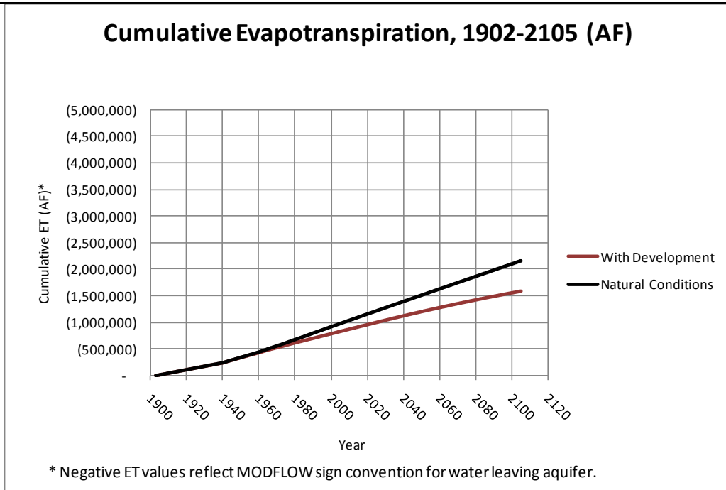
FIGURE 16. SIMULATED CUMULATIVE EVAPOTRANSPIRATION (AF) WITH AND WITHOUT HUMAN DEVELOPMENT FOR THE PERIOD 1902-2105.
