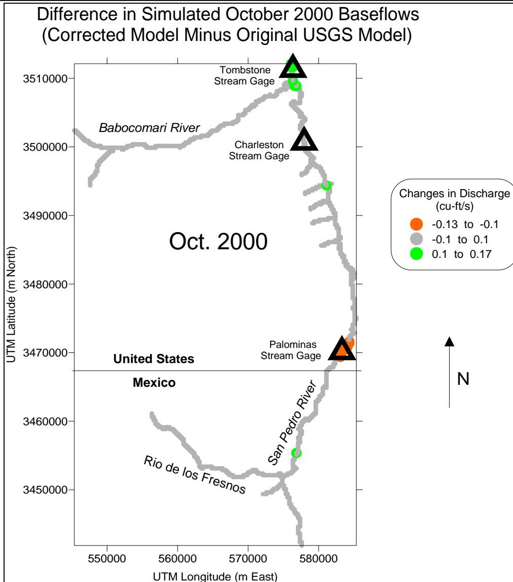
FIGURE 7. DIFFERENCE IN SIMULATED OCTOBER 2000 BASEFLOWS (CU-FT/S) AS COMPUTED BY SUBTRACTING ORIGINAL MODEL VALUES (POOL AND DICKINSON, 2007) FROM CORRECTED USGS MODEL VALUES. NEGATIVE CHANGE IN DISCHARGE VALUES INDICATES LOWER FLOWS AFTER MODEL CORRECTIONS; POSITIVE CHANGE IN DISCHARGE VALUES REPRESENTS HIGHER FLOWS AFTER CORRECTION.
