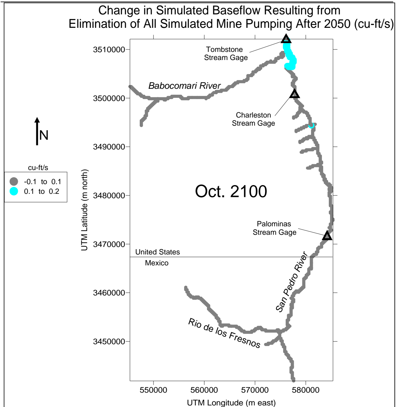
FIGURE 28. SIMULATED CHANGES IN BASEFLOW (CU-FT/S) AFTER DISCONTINUING MINE PUMPING NEAR CANANEA, MEXICO (SOUTH OF FIGURE BOUNDARY) AND NEAR BISBEE, ARIZONA (EAST OF FIGURE BOUNDARY JUST NORTH OF THE INTERNATIONAL BOUNDARY) AFTER 2050.
