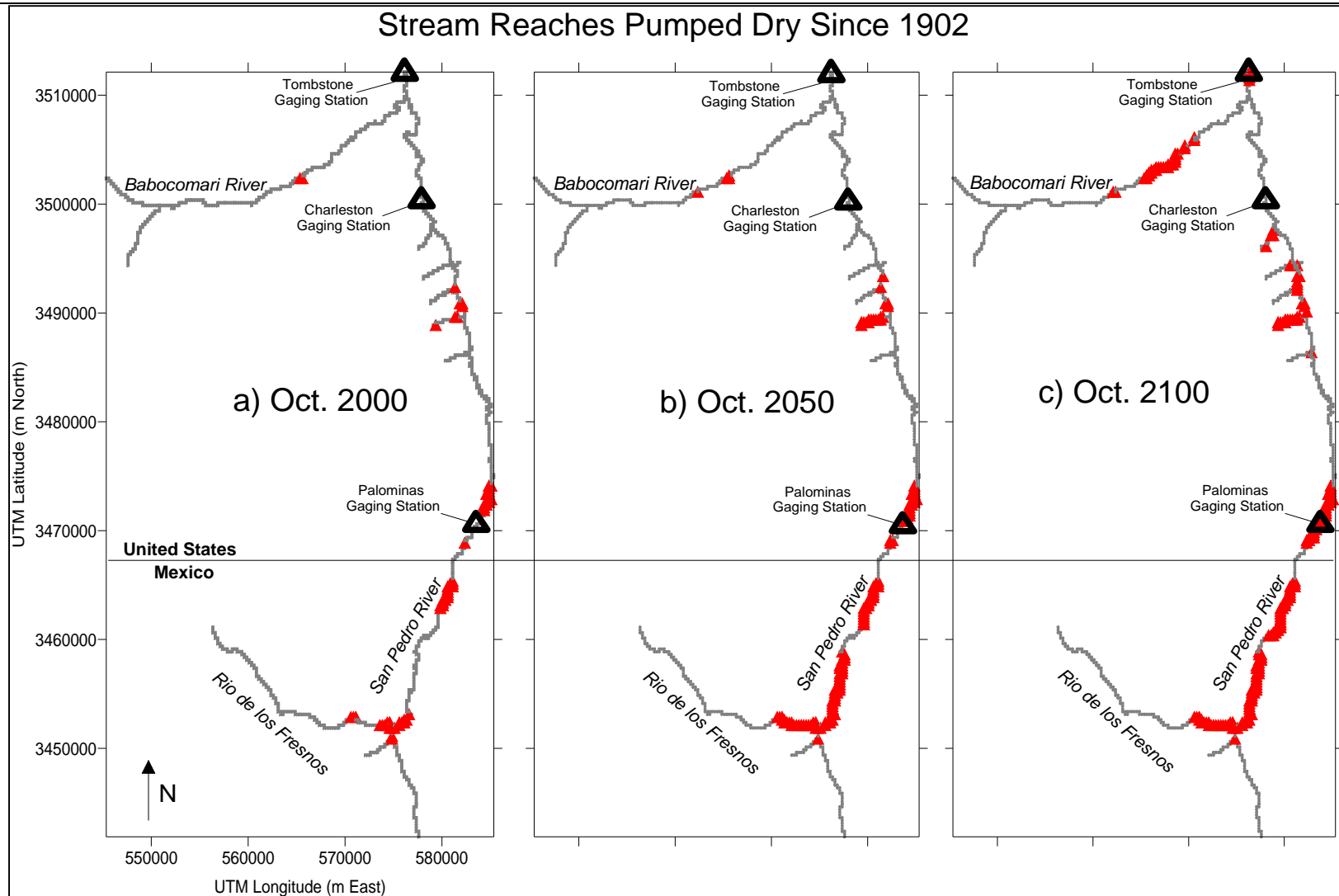
FIGURE 25. SIMULATED STREAM REACHES WITH NO FLOW AS A RESULT OF PUMPING IN: A) OCTOBER 2000, B) OCTOBER 2050, AND C) OCTOBER 2100. REACHES DRIED BY PUMPING ARE MARKED WITH RED TRIANGLES.
