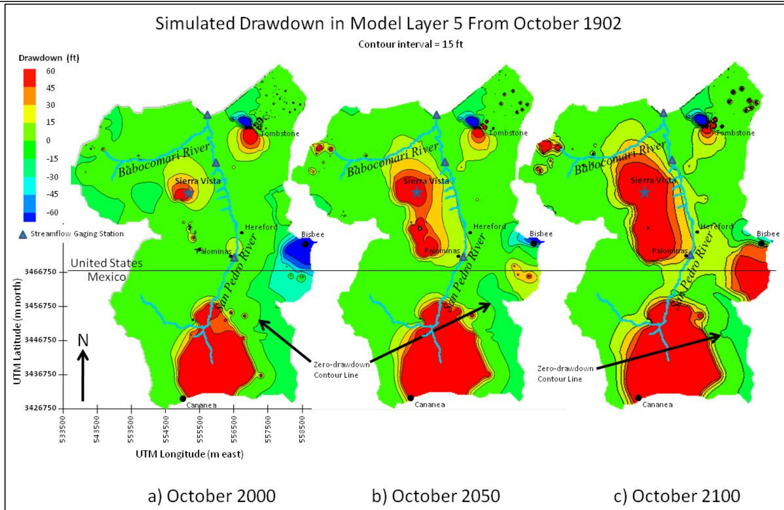
FIGURE 19. SIMULATED CHANGE IN HEAD (DRAWDOWN) (FT.) IN MODEL LAYER 5 (BASE OF REGIONAL AQUIFER) FROM OCTOBER 1902 TO OCTOBER 2000, OCTOBER 2050, AND OCTOBER 2100. AREAS IN DARK RED REPRESENT DRAWDOWN OF 60 FT. OR MORE. BLUE LINE REPRESENTS LOCATION OF RIVERS BUT DOES NOT SIGNIFY THE CONDITION OF PERENNIAL FLOW.
