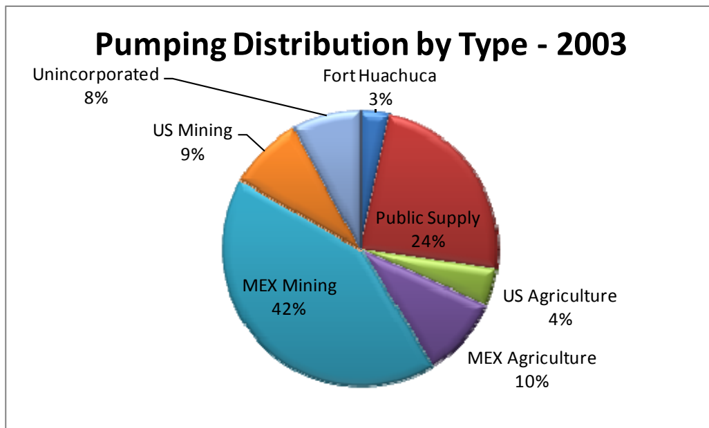
FIGURE 11. DISTRIBUTION OF SIMULATED PUMPING IN THE USBP BY TYPE AS OF MARCH 2003.
