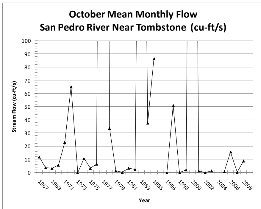
FIGURE 9. MEAN OCTOBER STREAM FLOW (CU-FT/S) ON THE SAN PEDRO RIVER MEASURED AT THE TOMBSTONE GAGING STATION FOR THE PERIOD OF RECORD, 1967-2008 (USGS, 2011). VERTICAL AXIS IS TRUNCATED AT 100 CU-FT/S TO HIGHLIGHT LOW FLOWS. 7
