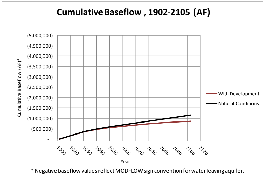
FIGURE 14. SIMULATED CUMULATIVE BASIN-WIDE BASEFLOW (AF) FOR THE PERIOD 1902-2105. THE RED CURVE INCLUDES PUMPING, ARTIFICIAL, AND INCIDENTAL RECHARGE WHILE THE BLACK CURVE REPRESENTS NATURAL CONDITIONS IN THE ABSENCE OF HUMAN DEVELOPMENT.
