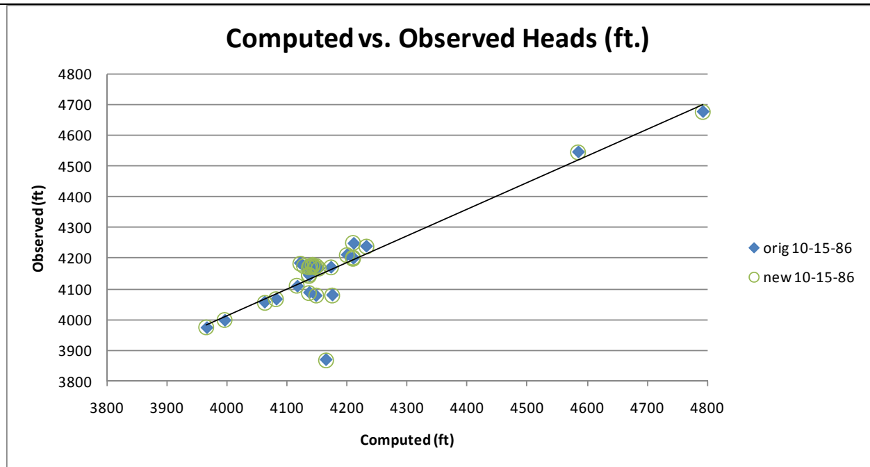
FIGURE 5. COMPUTED VS. OBSERVED HEADS (FT.) FOR OCTOBER 15, 1986 FOR THE ORIGINAL USGS MODEL (POOL AND DICKINSON, 2007) AND AFTER CORRECTIONS TO MODEL.
